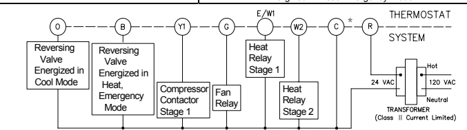
Figure 6. Typical wiring diagram for single transformer multi-stage systems
