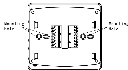
Figure 2. Thermostat base
